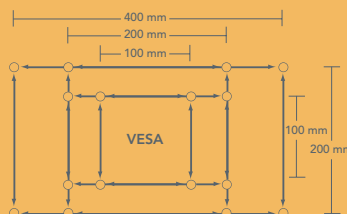
MSBV VESA Interface Bracket
