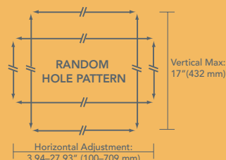
MSBU Universal Interface Bracket
