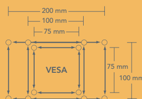
FSBV VESA Interface Bracket
