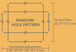
PSBU Universal Interface Bracket
